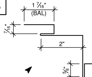
COLONIAL INSIDE CORNER (9" GIRTH)
