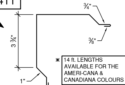
RAKE EDGE TRIM (12" GIRTH) (10 or 14 ft. LENGTHS) *
