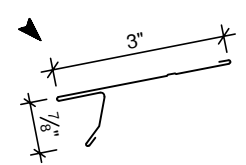
STARTER FOR SHINGLES (5" GIRTH)
