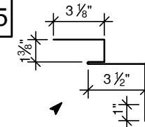
INSIDE CORNER (18" GIRTH)
