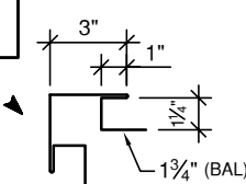
COMMERCIAL OUTSIDE CORNER (14" GIRTH)
