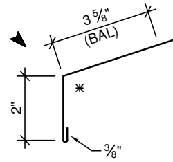
GUTTER APRON (6" GIRTH)
