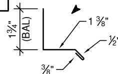
COMMERCIAL BASE FLASHING (4" GIRTH)
