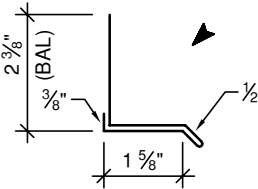
INDUSTRIAL WINDOW & DOOR FLASHING (7" GIRTH)
